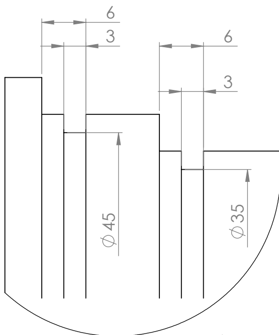
DETAIL B SCALE 2 : 1
